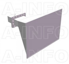
LB-770-15-C-SFSP0 Standard Gain Horn Antenna 0.96-1.45GHz 15dB Gain SMA Female
